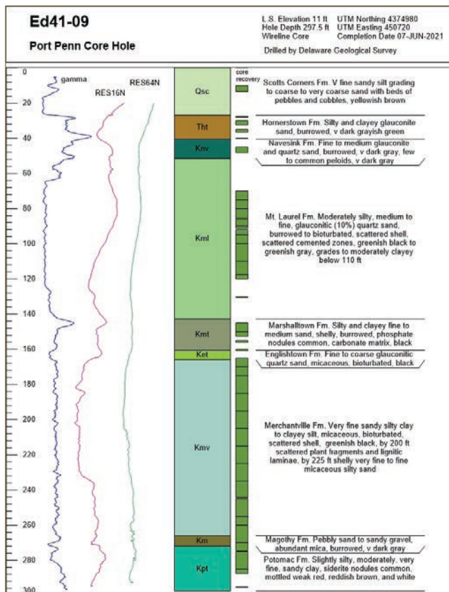
Example of standardized corehole log that displays essential geological data for key stratigraphic reference sections.
